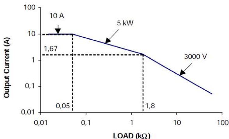
VIP 5000 LOAD LIMITS
