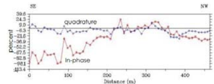
In-phase and quadrature VLF data (Transmitter 24.0 kHz. Cutler Maine, data used to produce the resistivity section above)
