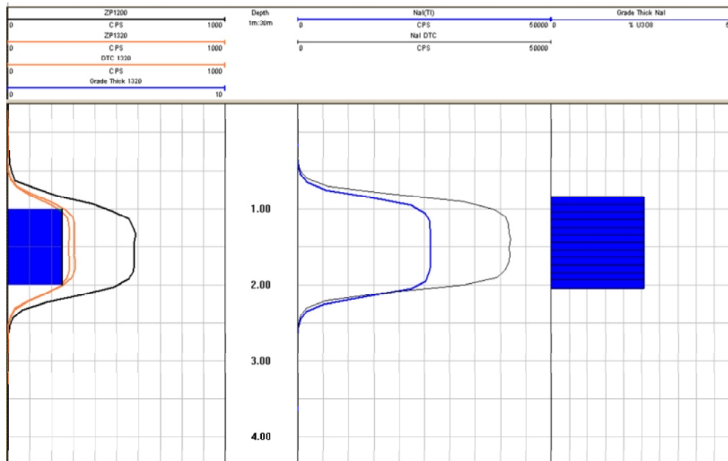
2GHF-1000 calibration in 2.6% U3O8 model
