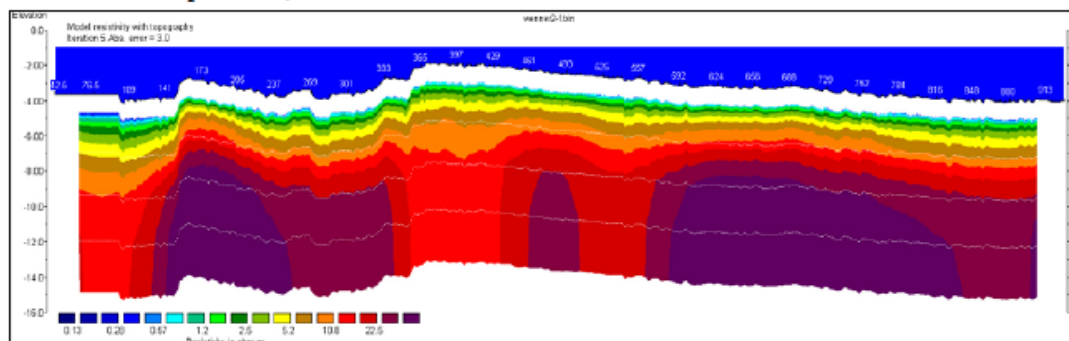
Interpreted marine resistivity section
