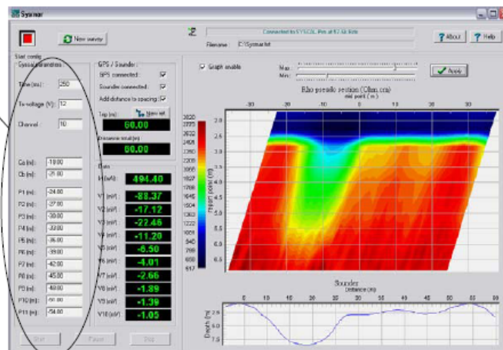
Real time resistivity pseudo-section picturing
