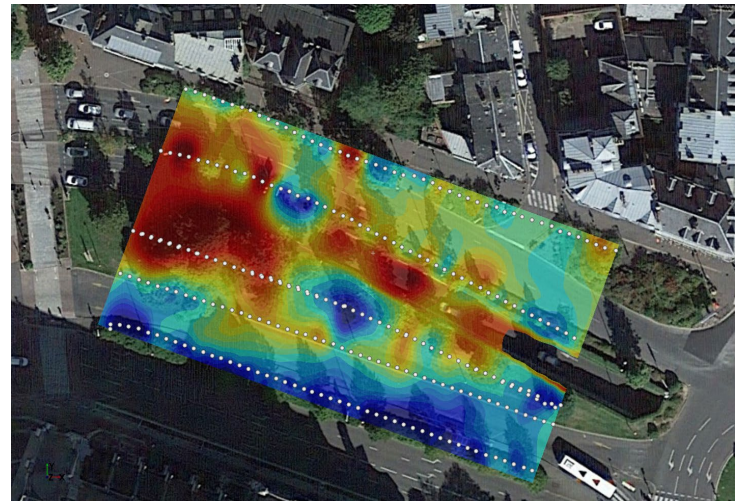
3D resistivity model obtained from the Multi-Tx survey
