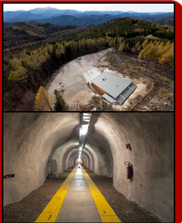
SuperGradiometer installed at Conrad Earth Observatory, Austria. (.02 pT sensitivity @ 1 Hz with <1pT noise level)
