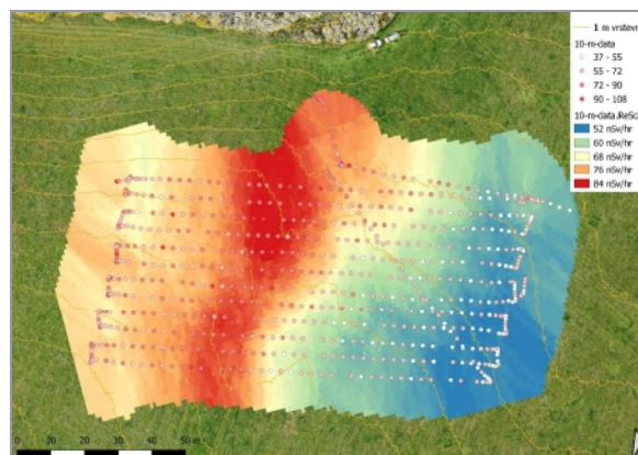
Contour Map of Dose Rate at 10m 1
