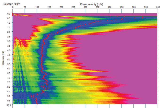
Dispersion curve for Atom array data acquired at the Lower 9th Ward site.
