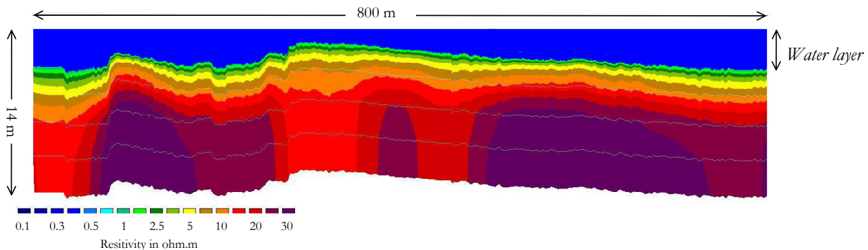
Inversed Resistivity section (3000 data points in 10 minutes)
