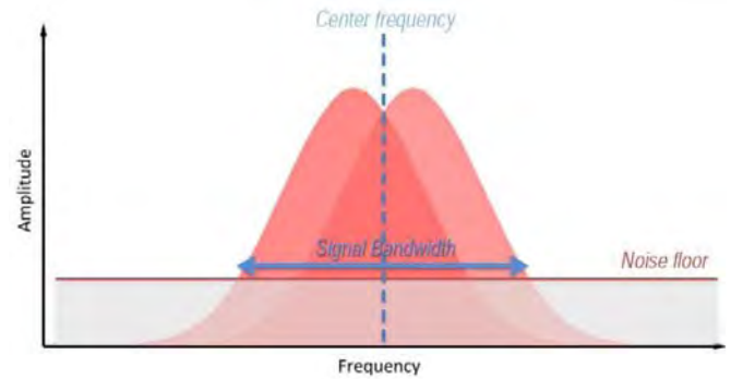
Typical conventional dual channel GPR System - Normal noise level, better bandwidth
